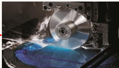
Wafer dicing
