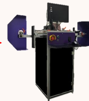
IV-200I Sorter/Counter
